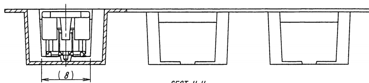
SECT. H-H
