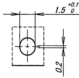
DETAIL J
