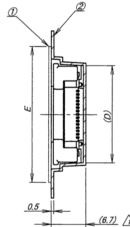
SECT. X-X
