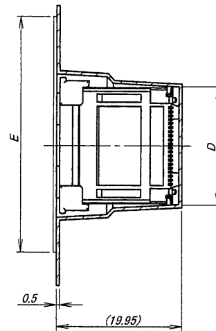
SECT. X-X
