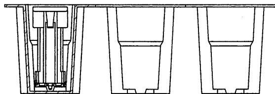
SECT. Y-Y
