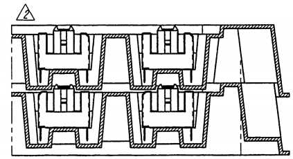
SECT B-B 梱包状態/PACKING CONDITION
