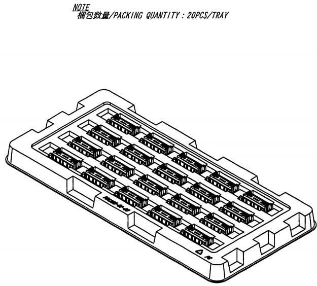
斜視図/ISOMETRIC VIEW
