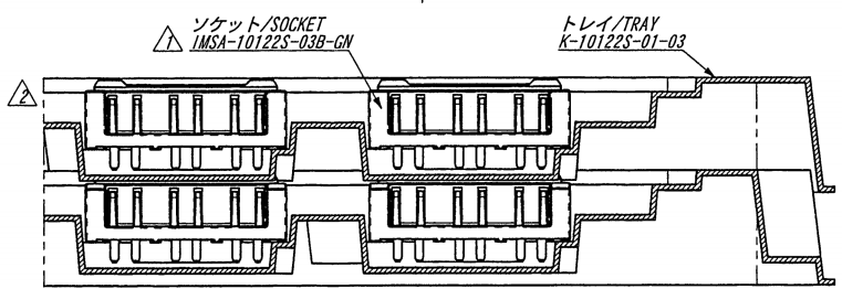
SECT A-A 梱包状態/PACKING CONDITION
