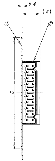
SECT. K-K
