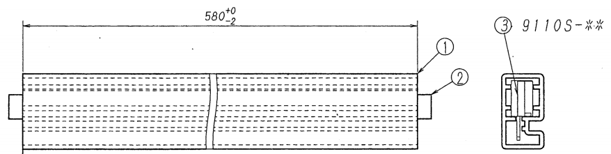
断面拡大図/SECT. DETAIL
