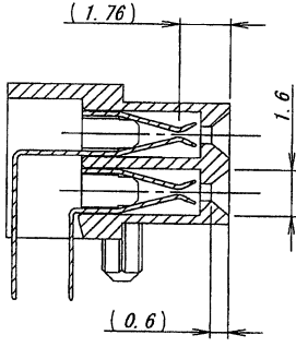
SECT B-B
