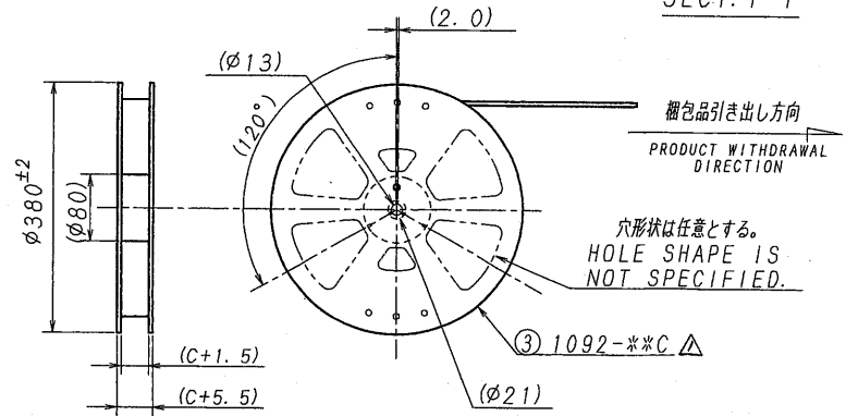
SECT. F-F
