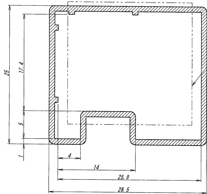
断面拡大図/SECT DETAIL
