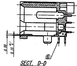
SECT. D-D
