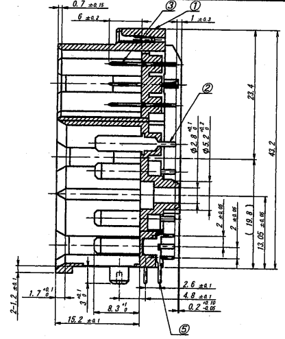
SECT. B-B
