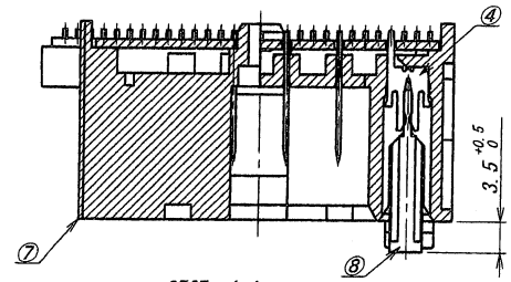
SECT. A-A
