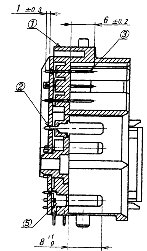
SECT. B-B
