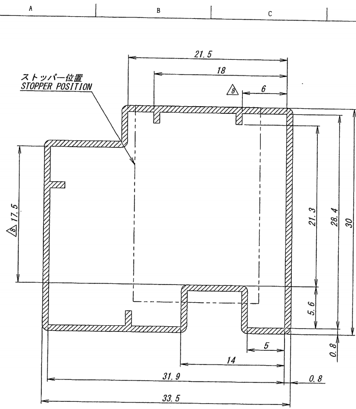
断面拡大図/SECT DETAIL
