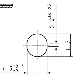
J 部詳細 (NOTE 4) SECTION J
