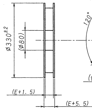
J 部詳細 (NOTE 4) SECTION J
