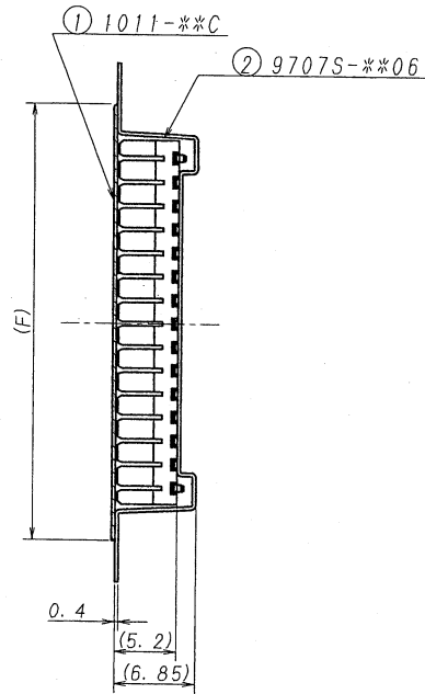
SECT G-G
