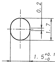
DETAIL J
