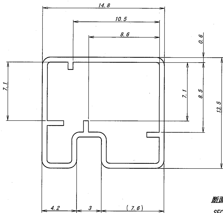
SECT. DETAIL
