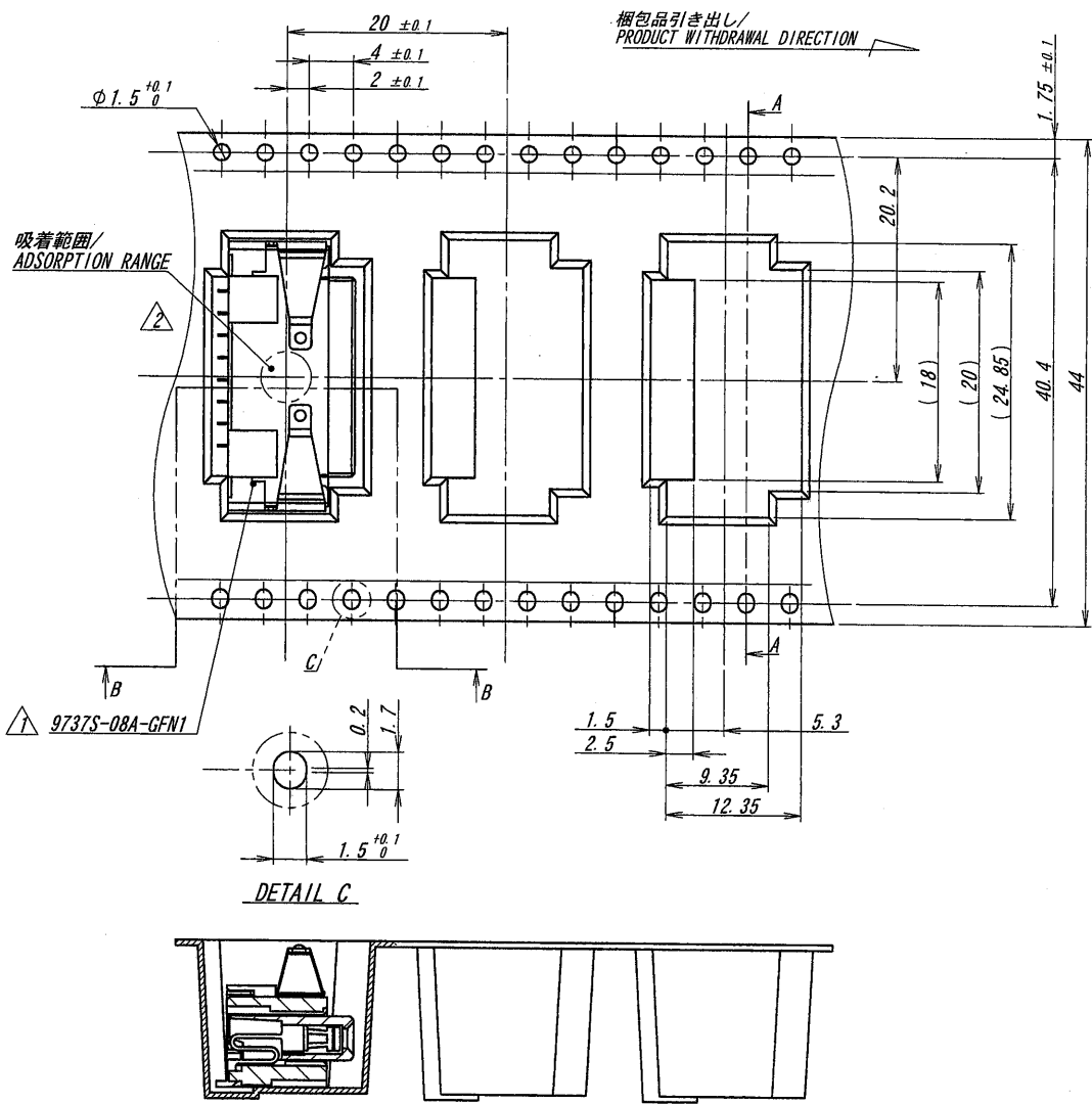
SECT B-B
