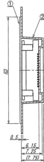
SECT. H-H
