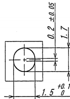
DETAIL K
