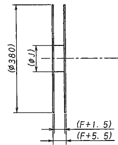
SECT H-H
