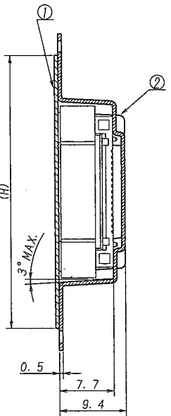
SECT H-H
