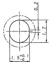
DETAIL K
