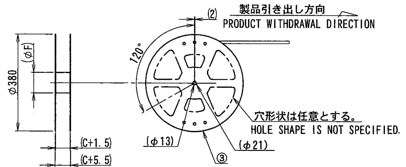
SECT. Y-Y
