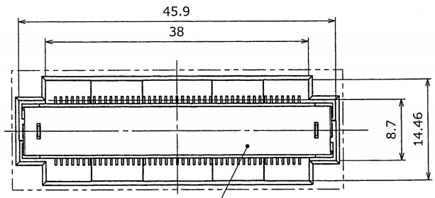
②9828S-90Z07-GFN4 DETAIL A
