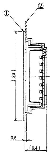
SECT. A-A
