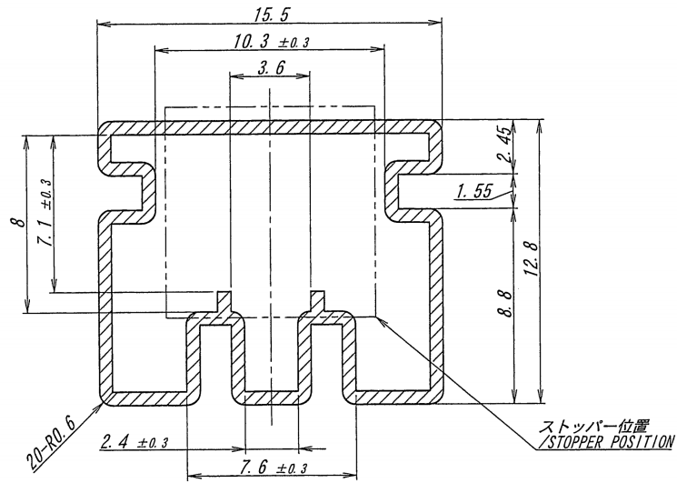
断面拡大図/SECT. DETAIL
