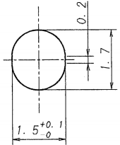
DETAIL K (NOTE 4)
