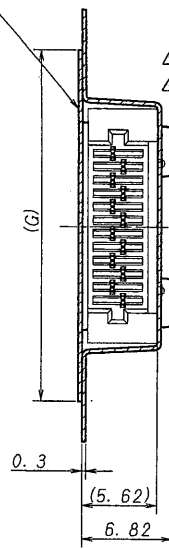
SECT. H-H
