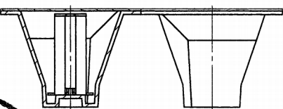
SECT. F-F
