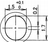
DETAIL H
