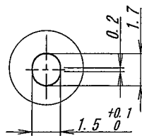
DETAIL K
