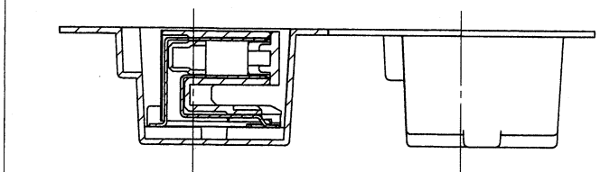
SECT. H-H
