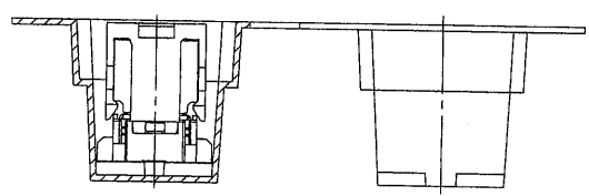
SECT. H-H
