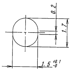
DETAIL J
