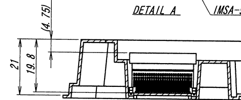
SECT. C-C
