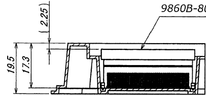
SECT. B-B
