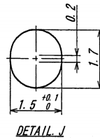
DETAIL J
