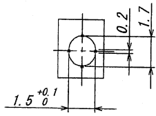
DETAIL J
