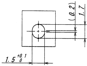
DETAIL "J"
