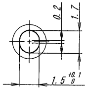
DETAIL. Z
