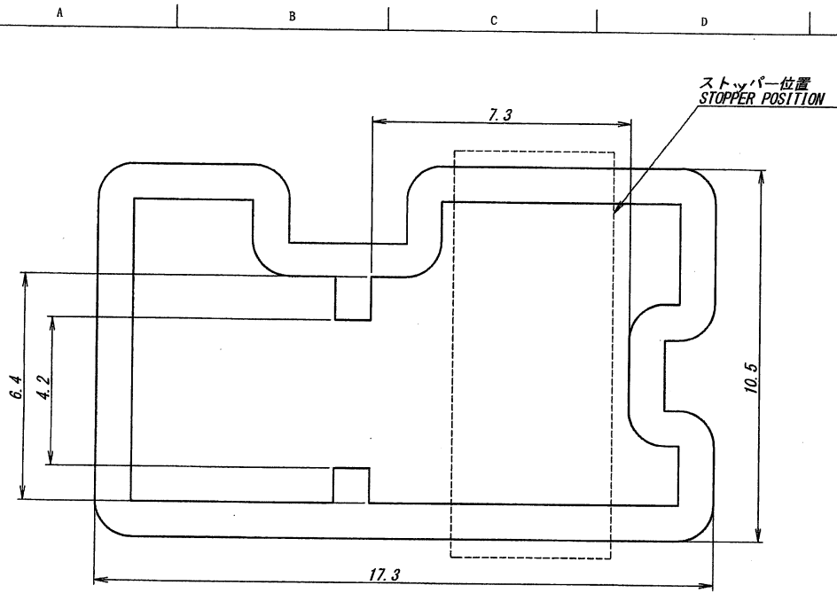
断面拡大図/SECT DETAIL
