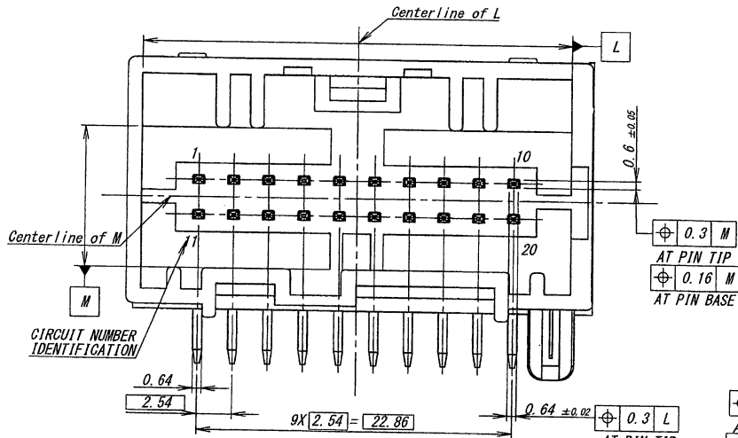
DETAIL H
