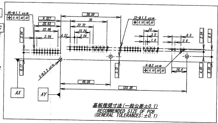
DETAIL J
