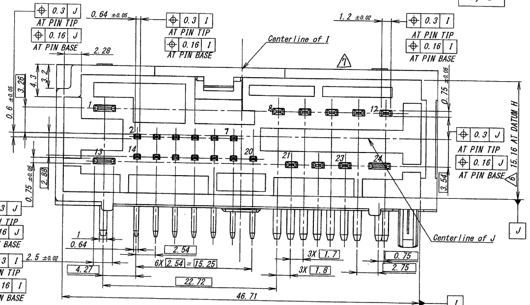
DETAIL J
