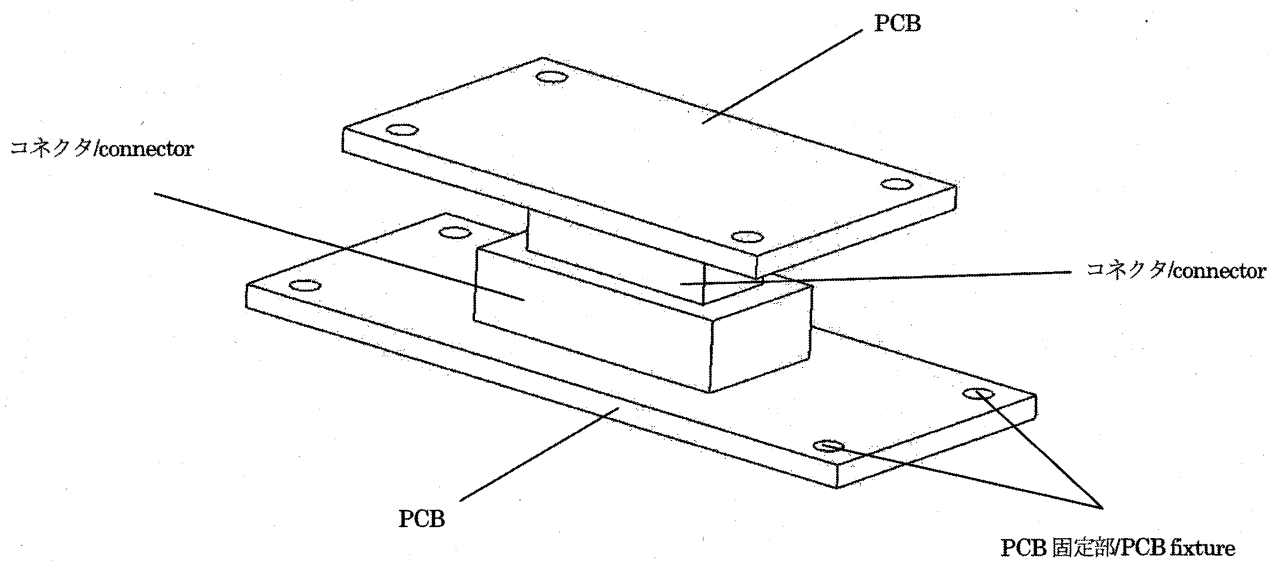
平行接続/parallel connection
