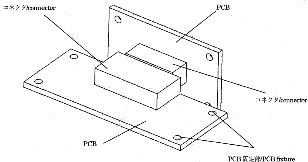
垂直接続/vertically connection
